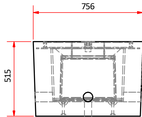
END VIEW ( 1:15 )
